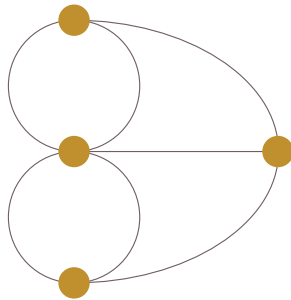
The image at the top appeared in the original paper by Euler in 1736, and it shows the seven bridges in the city of Königsberg. The diagram at the bottom depicts the same problem as a graph.
